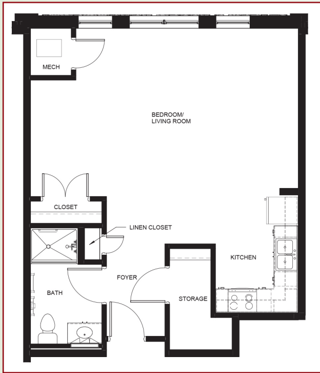
Studio Apartment
